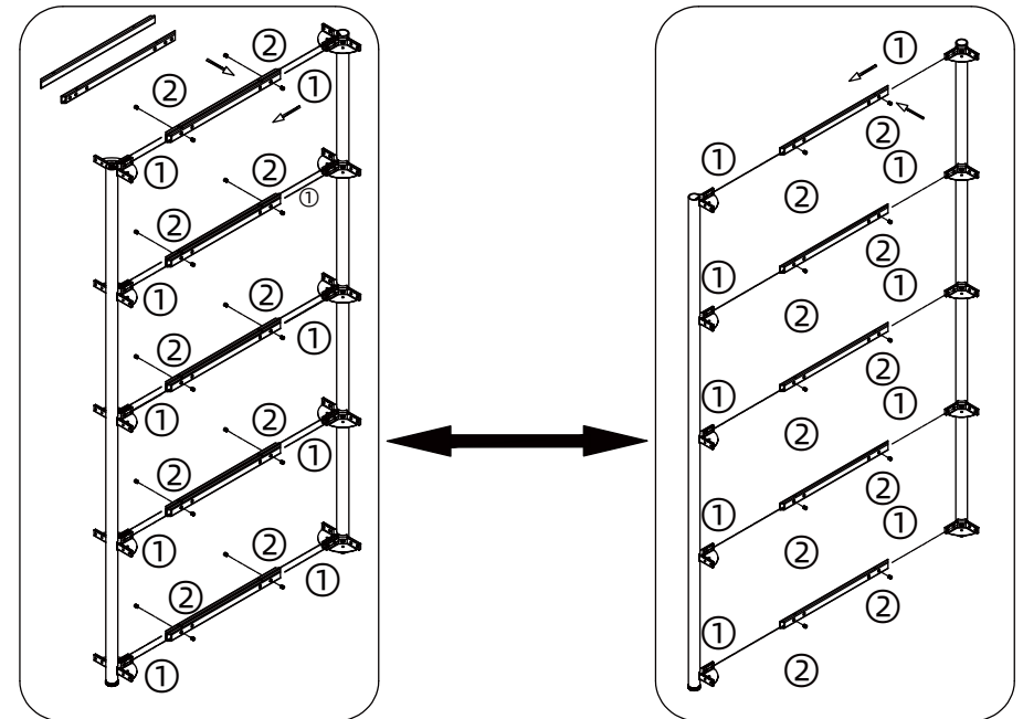
Install Intermediate Uprights and Beams
