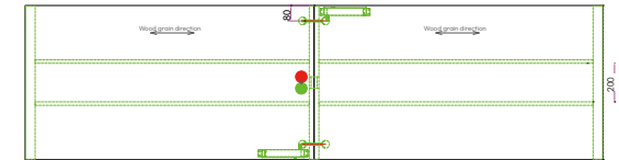
Socket Layout and Wiring Diagram for Double-Sided Segmented Bar Counter
