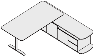
KAY-HAT-Semi-veneer/All-panel XXL: 2150*2130*750-1290 XL-A: 1950*2130*750-1290 XL-B: 1950*1830*750-1290 L: 1750*1830*750-1290
