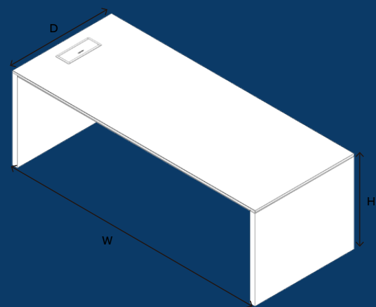
Econ top table (standard type/solid wood type) W=1800/2000/2200/2400 D=900/1000 H=750
