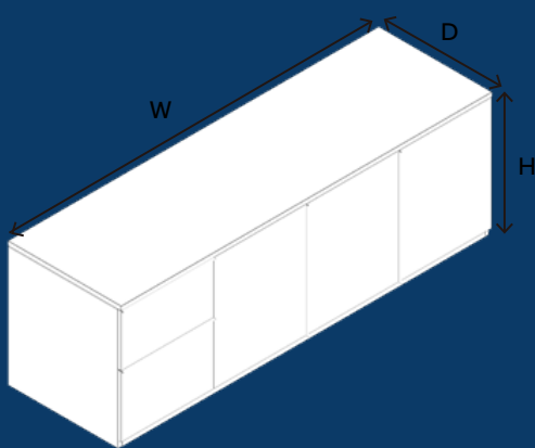
Econ side cabinet (solid wood type) W=1400 D=520 H=609
